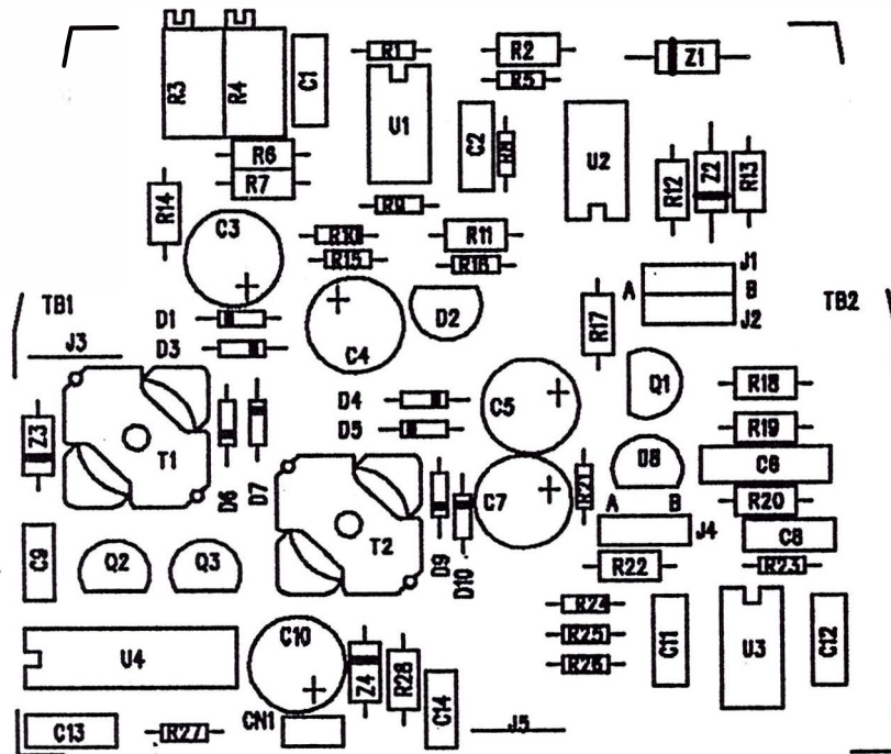
COMPONENT ASSEMBLY
